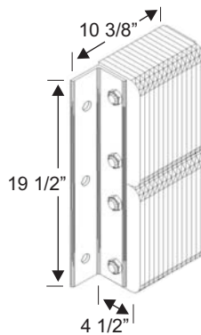
Model VB420-11F
